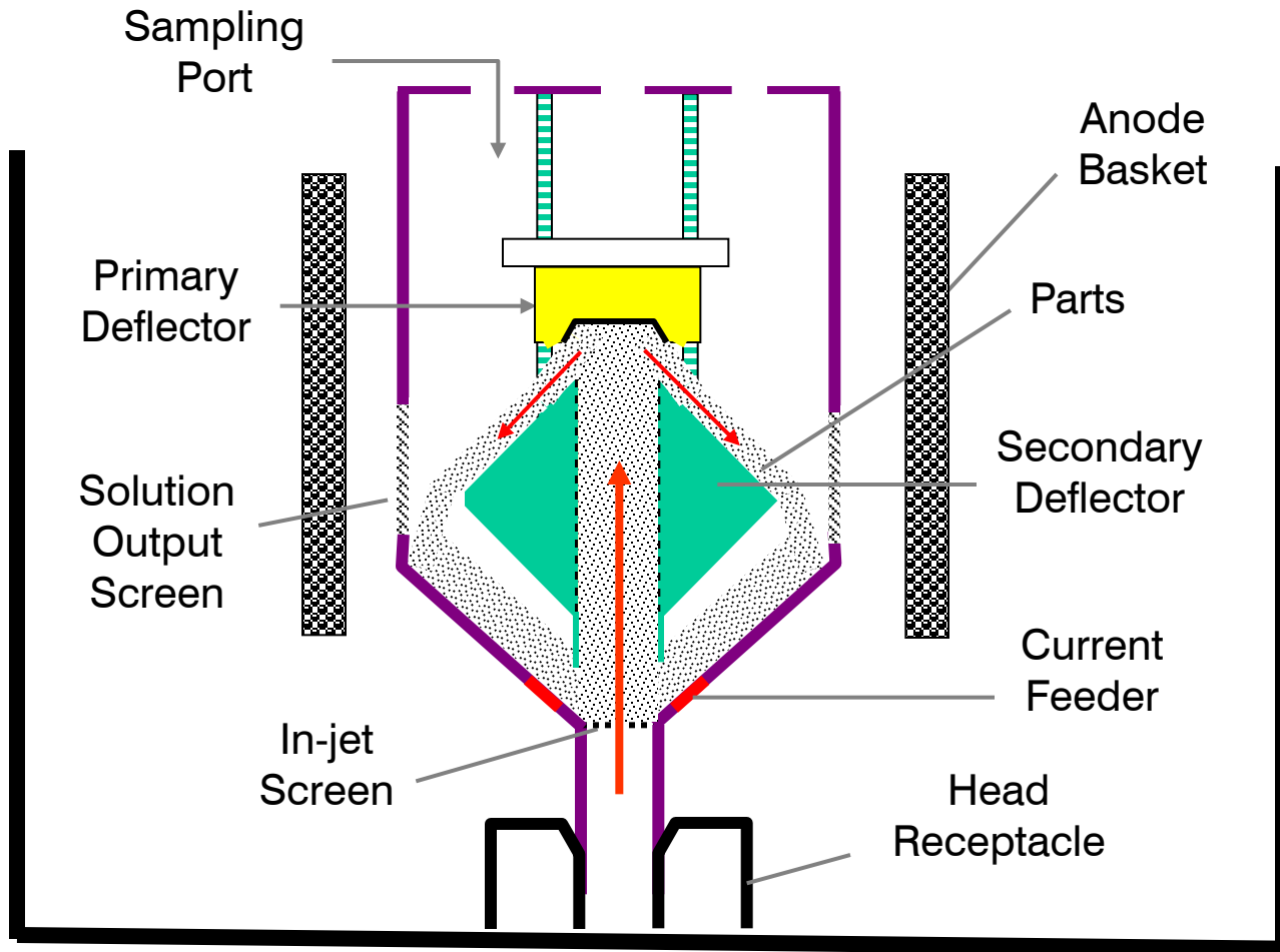
Plating Cell
