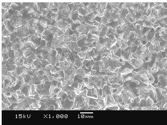
18 micron thickness
