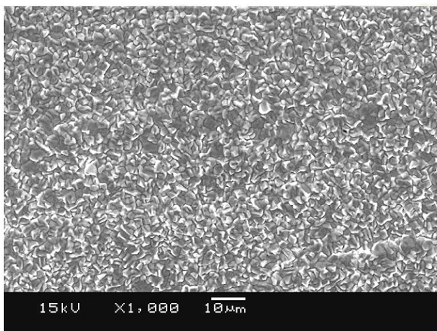
4 micron thickness
